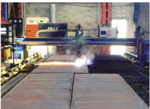
> 数控精细等离子切割机 (出口缅甸) CNC Precise plasma cutting machine to burma
