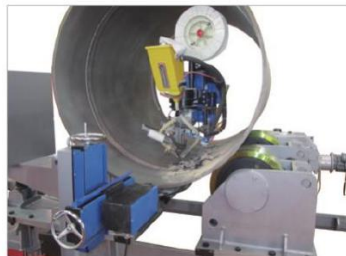
> 内环缝焊接 Inner seam welding
